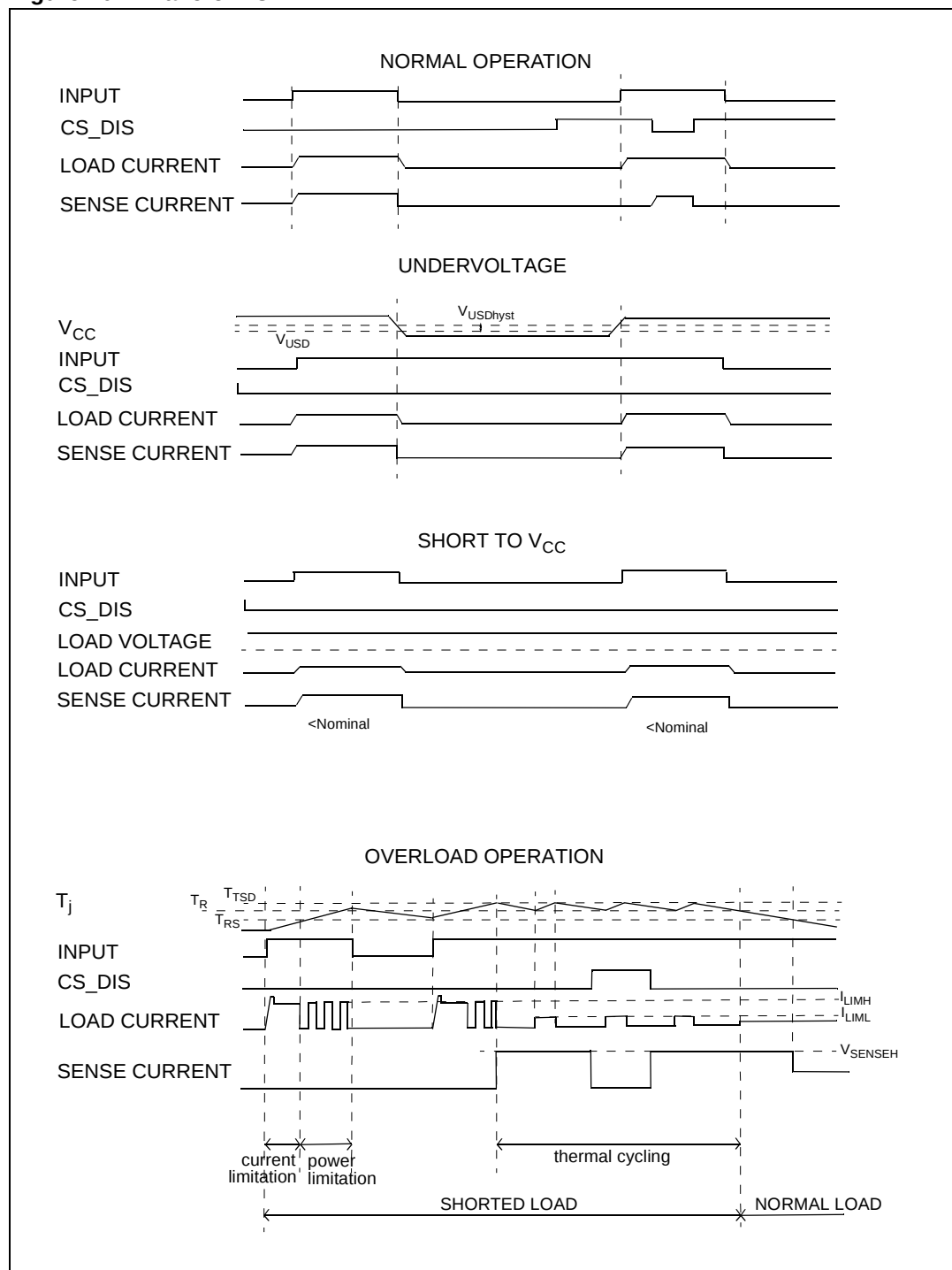
Figure 10. Waveforms
