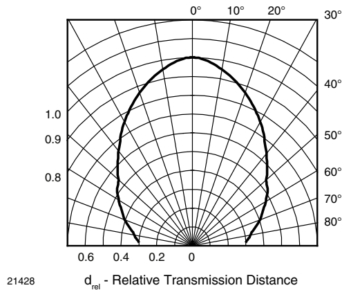
Fig. 10 - Vertical Directivity
