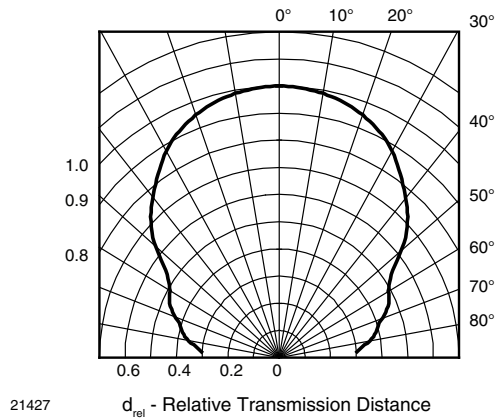
Fig. 9 - Horizontal Directivity
