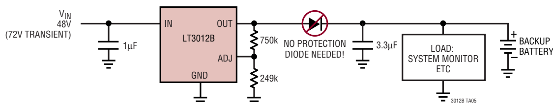
LT3012B Telecom Application
