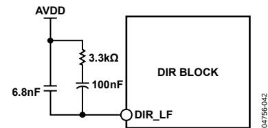
Figure 42. DIR Loop Filter Components
