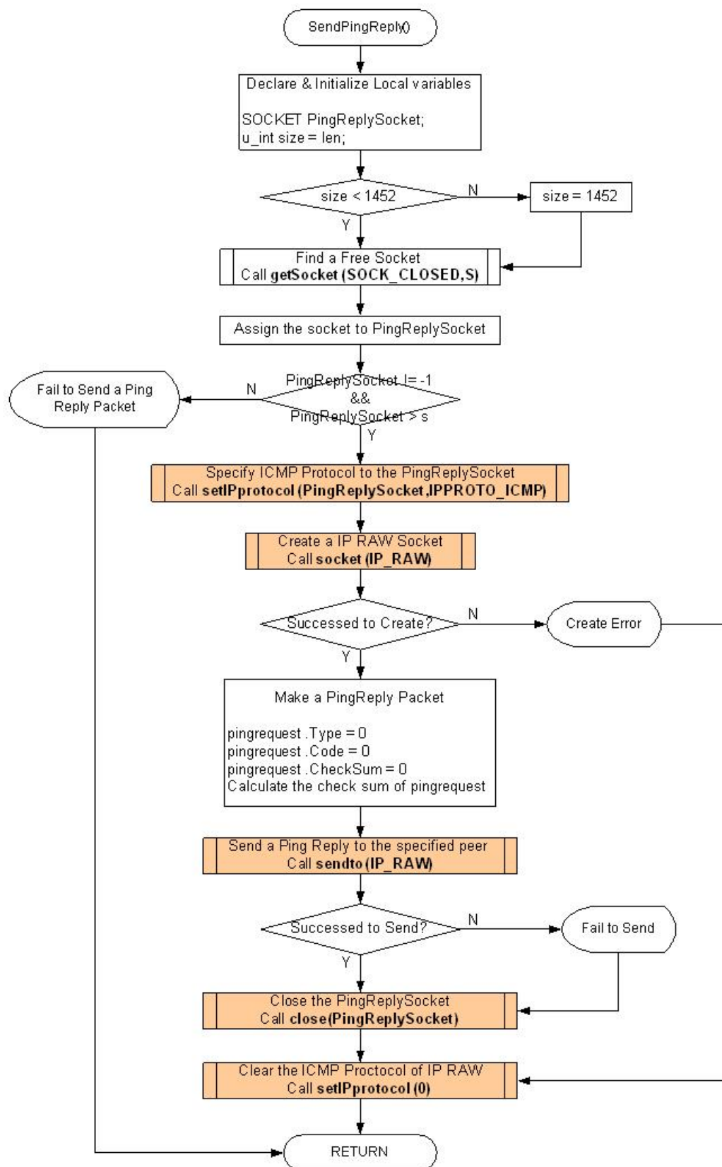
<Fig 3.13: SendPingReply()>
