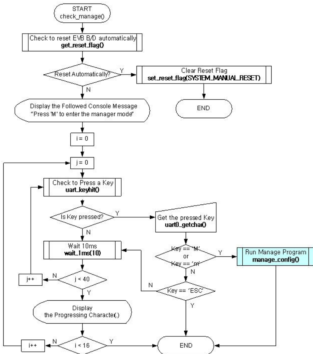
<Fig 3.4: check_manage()>
