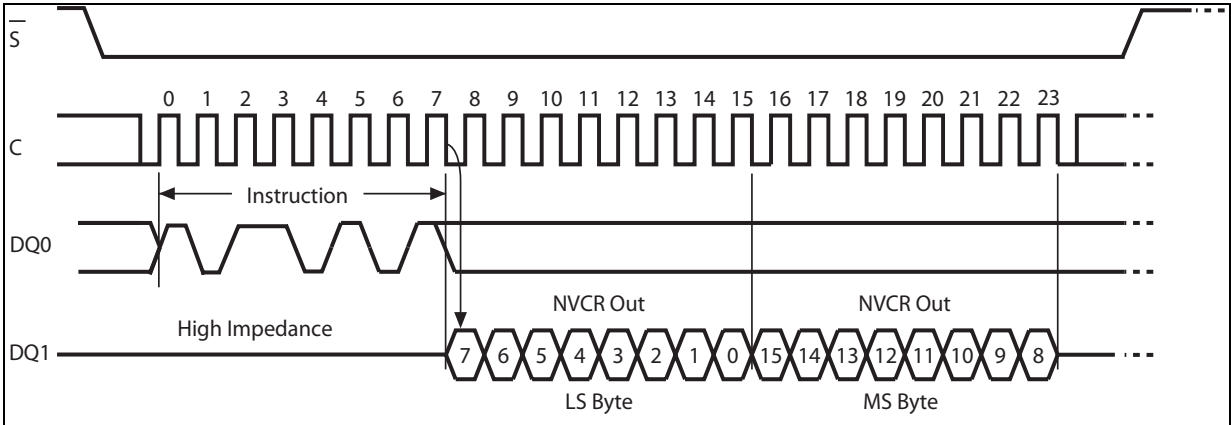
Figure 37. Read NV Configuration Register instruction sequence
