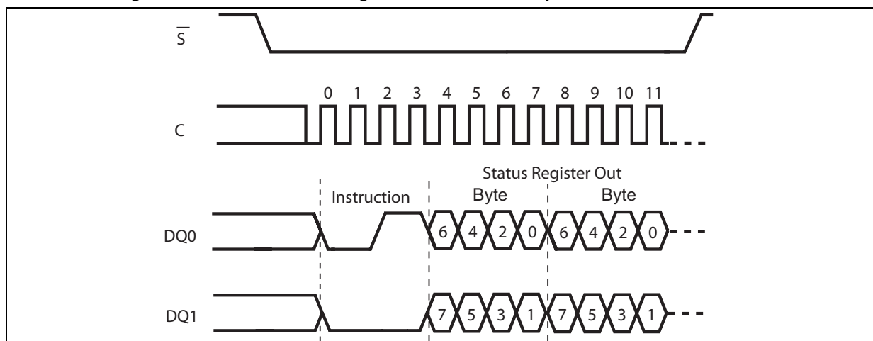
Figure 59. Read Status Register instruction sequence DIO-SPI
