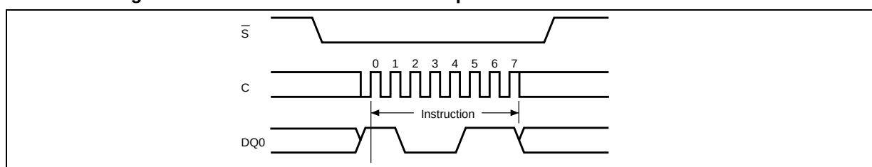
Figure 30. Bulk Erase instruction sequence
