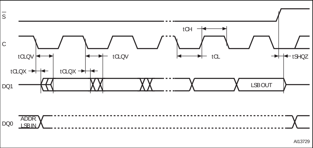
Figure 111. Output timing
