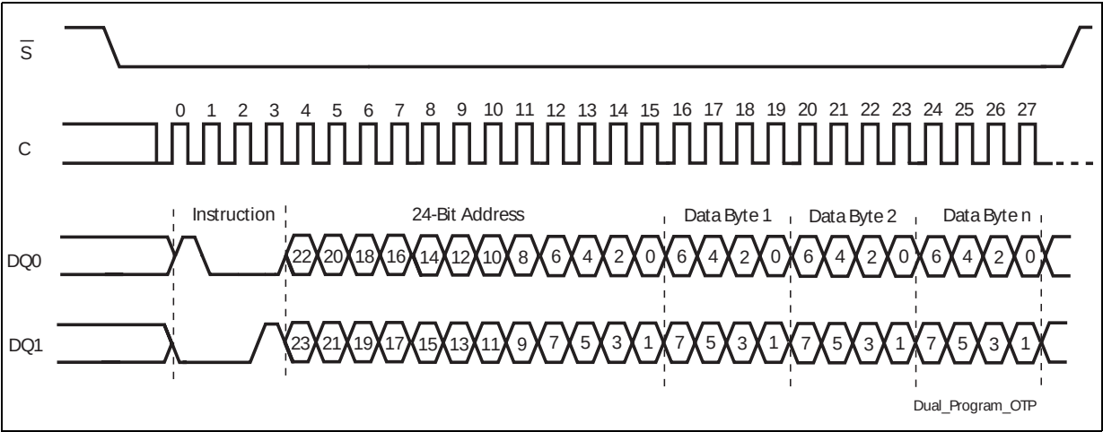
Figure 53. Program OTP instruction sequence DIO-SPI
