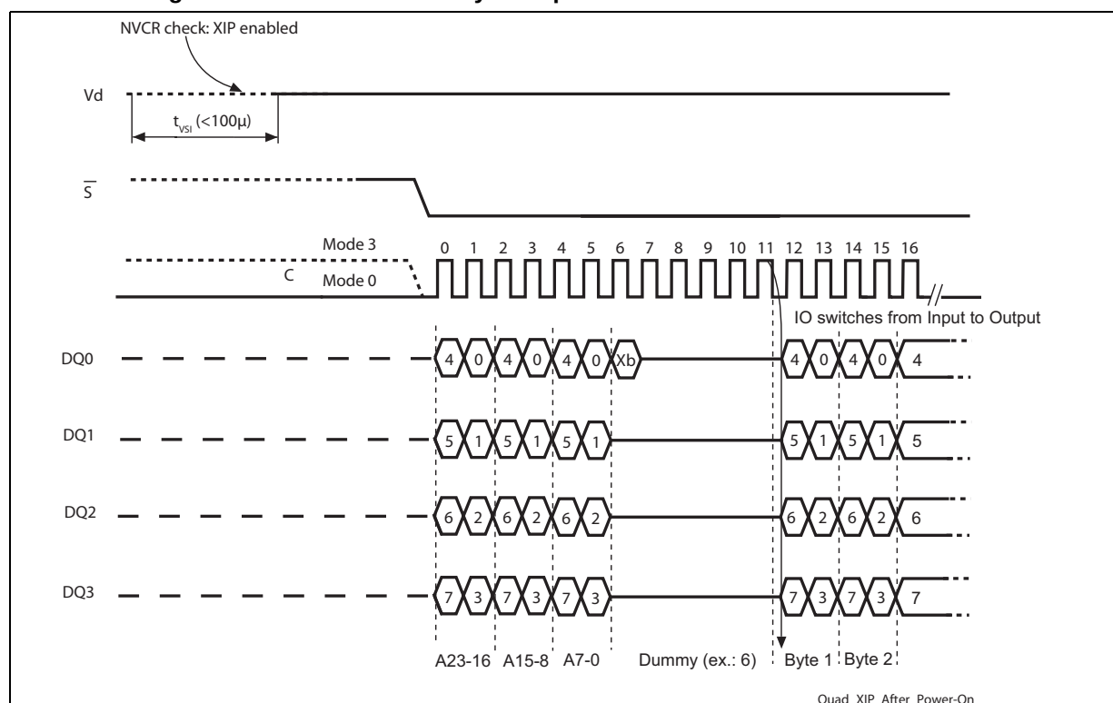
Figure 103. XIP mode directly after power on
