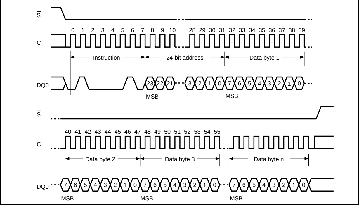
Figure 27. How to permanently lock the OTP bytes
