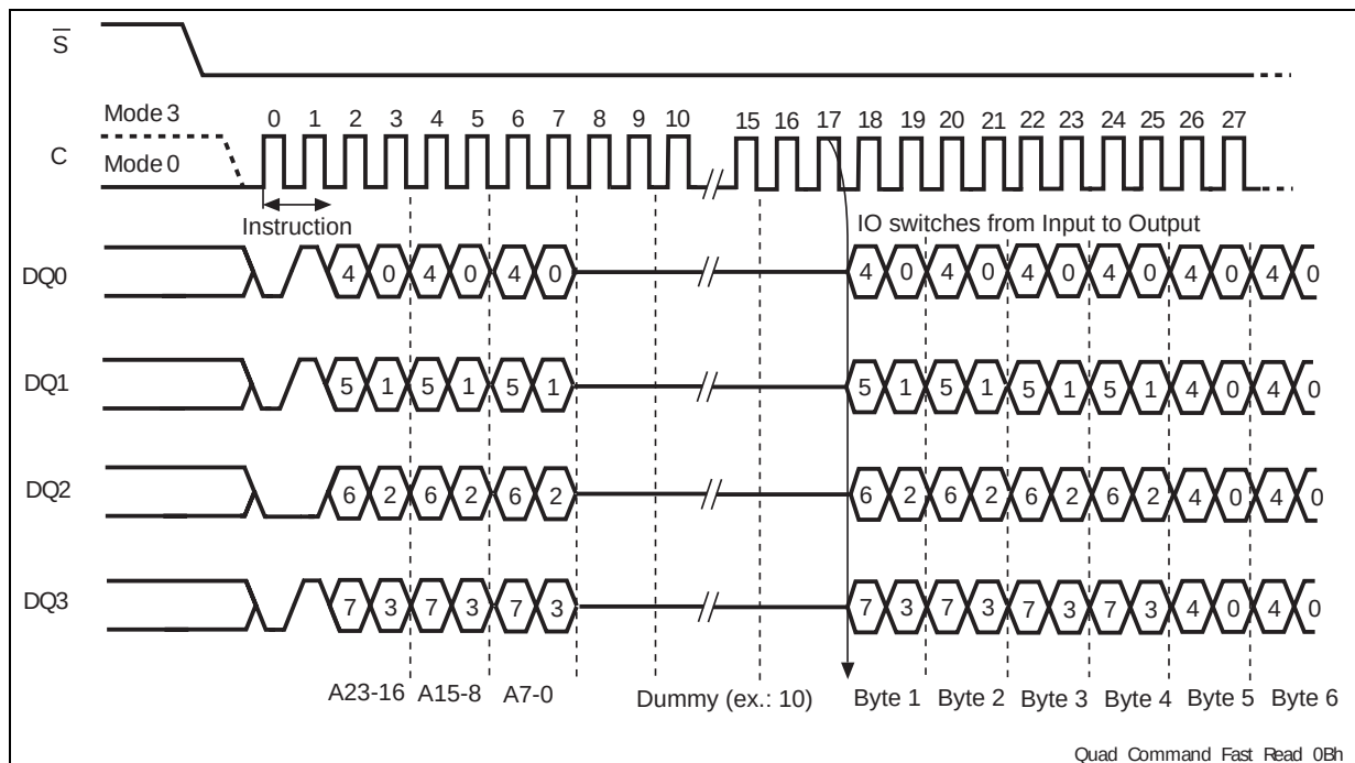
Figure 74. Quad Command Fast Read instruction and data-out sequence QIO-SPI, 0Bh
