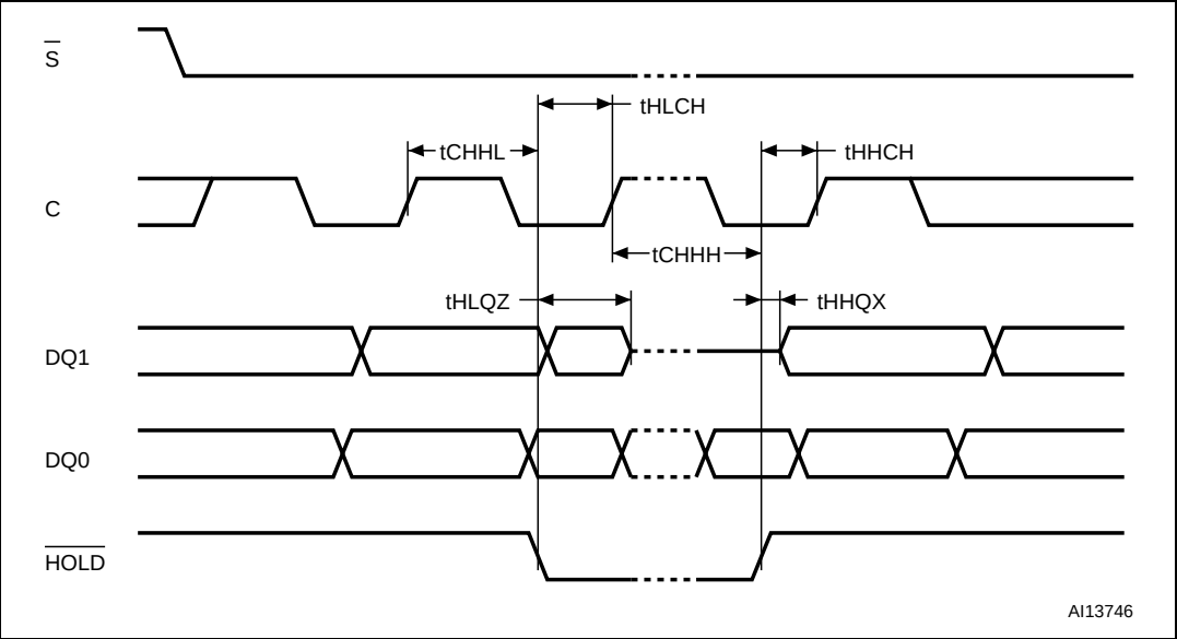
Figure 110. Hold timing
