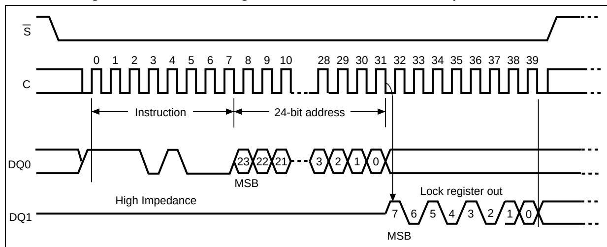
Figure 33. Read Lock Register instruction and data-out sequence
