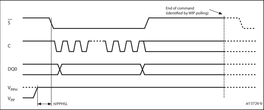
Figure 112. V_{PPH} timing
