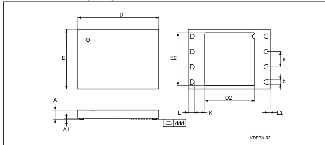
Figure 113. VDFPN8 (MLP8) Very thin Dual Flat Package No lead, 8 × 6 mm, package outline
