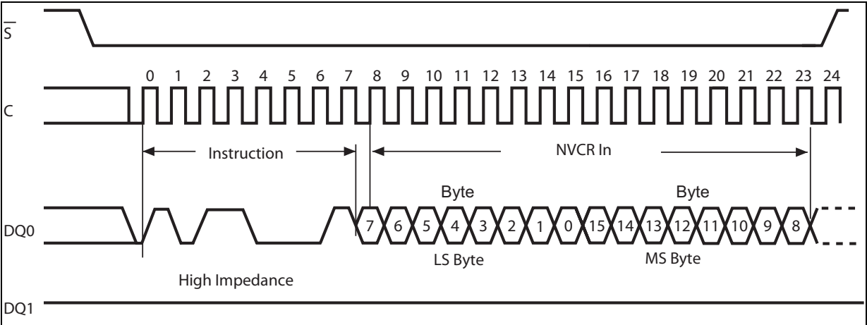
Figure 38. Write NV Configuration Register instruction sequence
