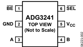
Figure 2. 6-Lead SC70
