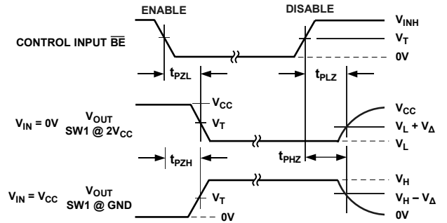
Figure 26. Enable and Disable Times
