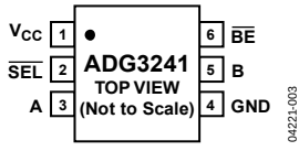
Figure 3. 6-Lead SOT-66
