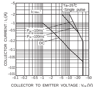
Fig.9 Safe operation area (2SB1237)
