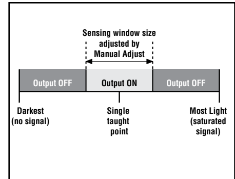
Figure 4. Single-Point TEACH (Light Operate shown)
