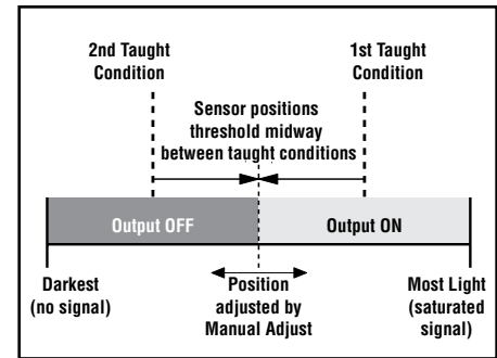
Figure 2. Two-Point TEACH (Light Operate shown)
