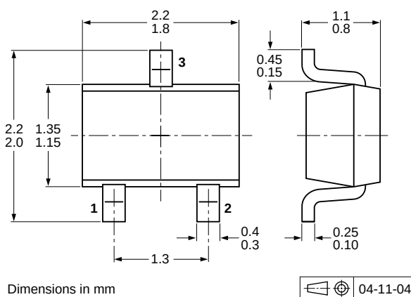
Fig 15. Package outline PDTC143ZU (SOT323/SC-70)
