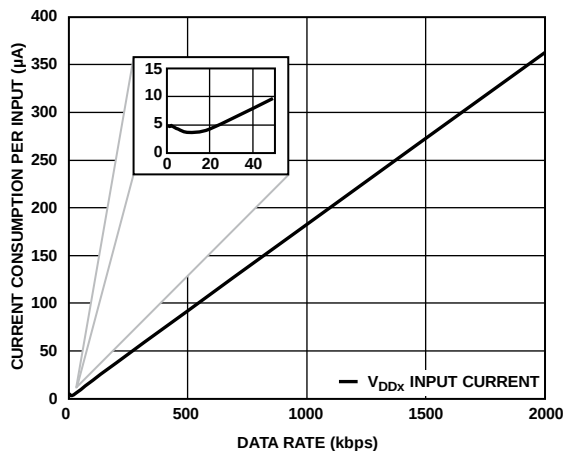
Figure 9. Current Consumption per Input vs. Data Rate for 3.3 V, EN_x = Low Operation
