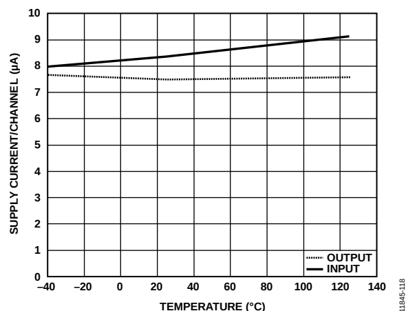
Figure 18. Typical Input and Output Supply Current per Channel vs. Temperature for V_{DDX} = 3.3\text{ V} , Data Rate = 100 kbps
