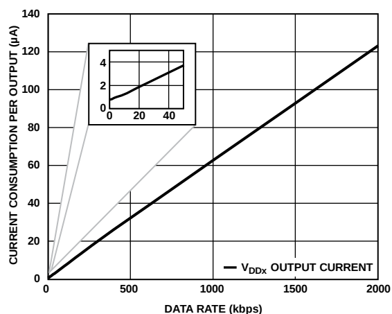
Figure 10. Current Consumption per Output vs. Data Rate for 3.3 V, EN_x = Low Operation
