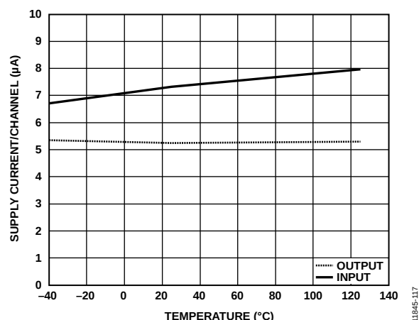
Figure 17. Typical Input and Output Supply Current per Channel vs. Temperature for V_{DDX} = 2.5\text{ V} , Data Rate = 100 kbps
