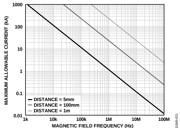
Figure 28. Maximum Allowable Current for Various Current-to-ADuM144x Spacings
