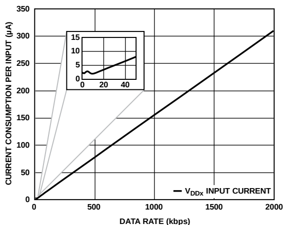
Figure 7. Current Consumption per Input vs. Data Rate for 2.5 V, EN_x = Low Operation
