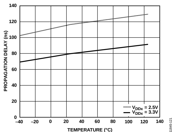
Figure 21. Typical Propagation Delay vs. Temperature for V_{DDx} = 3.3 V or V_{DDx} = 2.5 V
