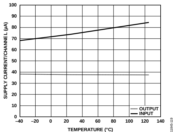
Figure 19. Typical Input and Output Supply Current per Channel vs. Temperature for V_{DDx} = 2.5 V, Data Rate = 1000 kbps
