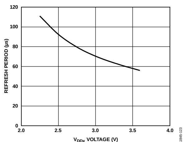
Figure 24. Typical Refresh Period vs. V_{DDx} Voltage
