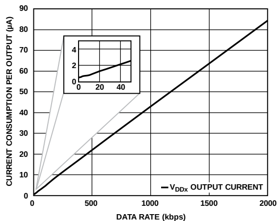
Figure 8. Current Consumption per Output vs. Data Rate for 2.5 V, EN_x = Low Operation
