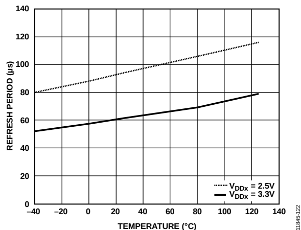
Figure 23. Typical Refresh Period vs. Temperature for 3.3 V and 2.5 V Operation
