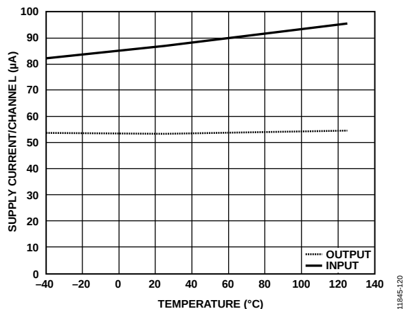
Figure 20. Typical Input and Output Supply Current per Channel vs. Temperature for V_{DDx} = 3.3 V, Data Rate = 1000 kbps
