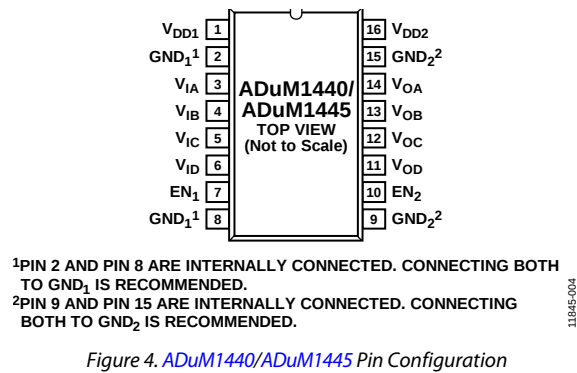
Figure 4. ADuM1440/ADuM1445 Pin Configuration
