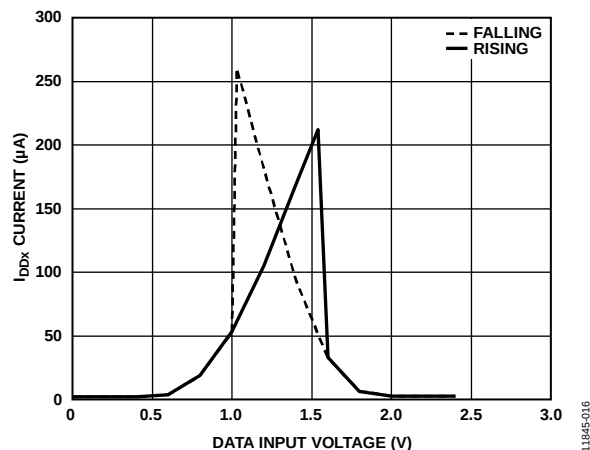
Figure 16. I_{DDX} Current per Input vs. Data Input Voltage for V_{DDX} = 2.5\text{ V}
