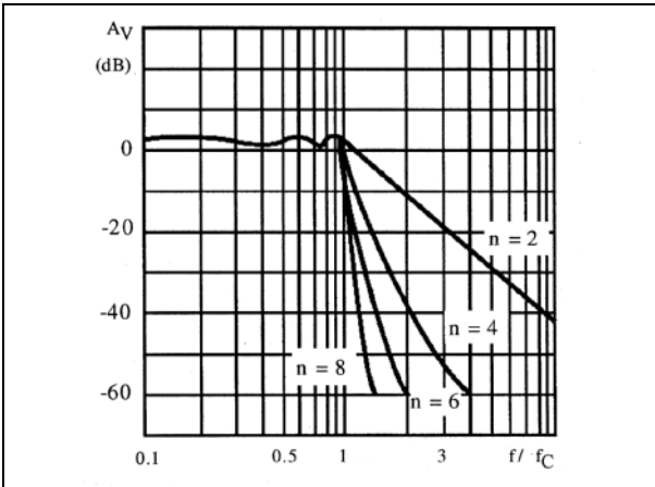
Figure 12. Amplitude response ( \pm 1\text{dB} ripple)
