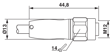
Dimensioned drawing
