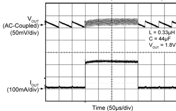
Load Transient (10mA to 200mA)
