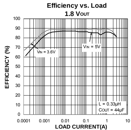
Figure 2. Efficiency Under Load
