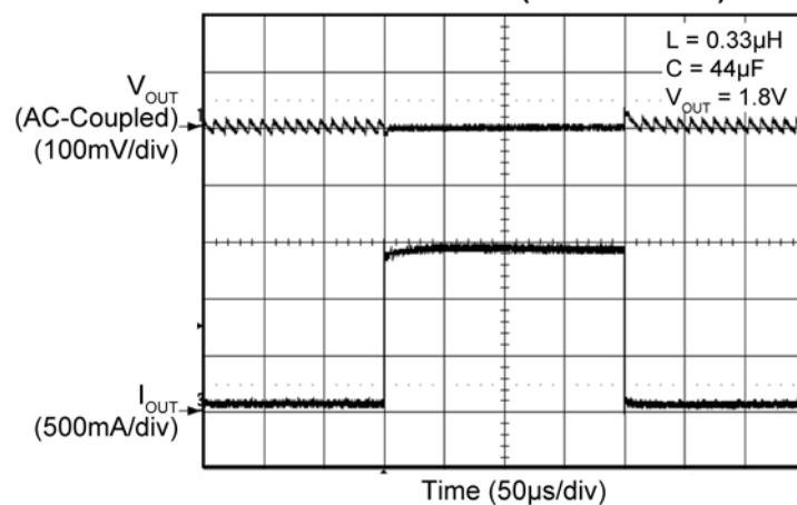
Load Transient (50mA to 1.5A)
