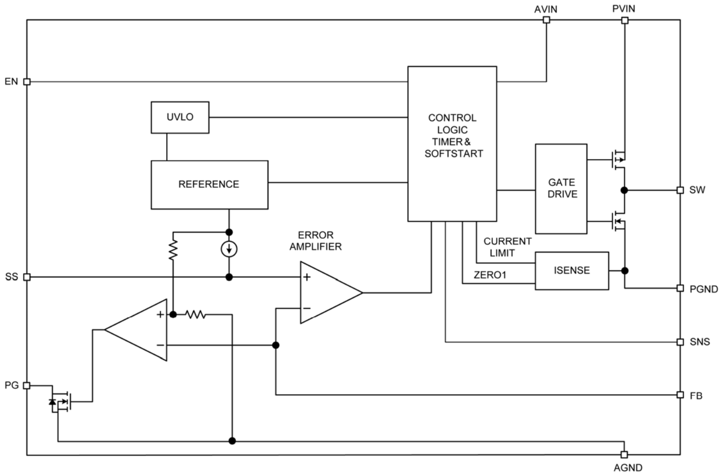
Figure 1. Simplified MIC23303 Functional Block Diagram
