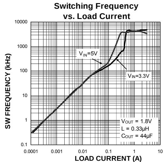
Figure 3. SW Frequency vs. Output Current
