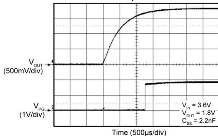
Start-Up PGOOD
