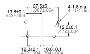
(Copper-side view)
