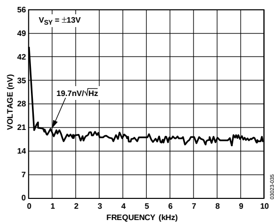
Figure 35. Voltage Noise Density
