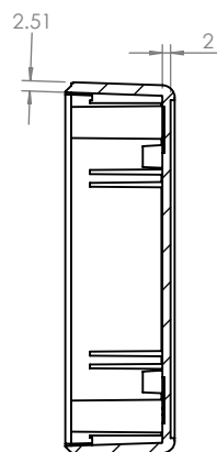
SECTION B-B
