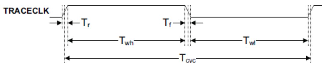
Figure 5. TRACE_CLKOUT specifications
