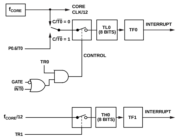
Figure 101. Timer/Counter 0, Mode 3
