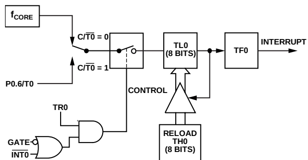
Figure 100. Timer/Counter 0, Mode 2
