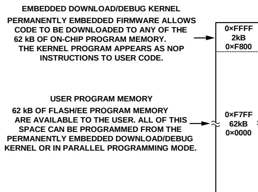
Figure 93. Flash Memory Organization
