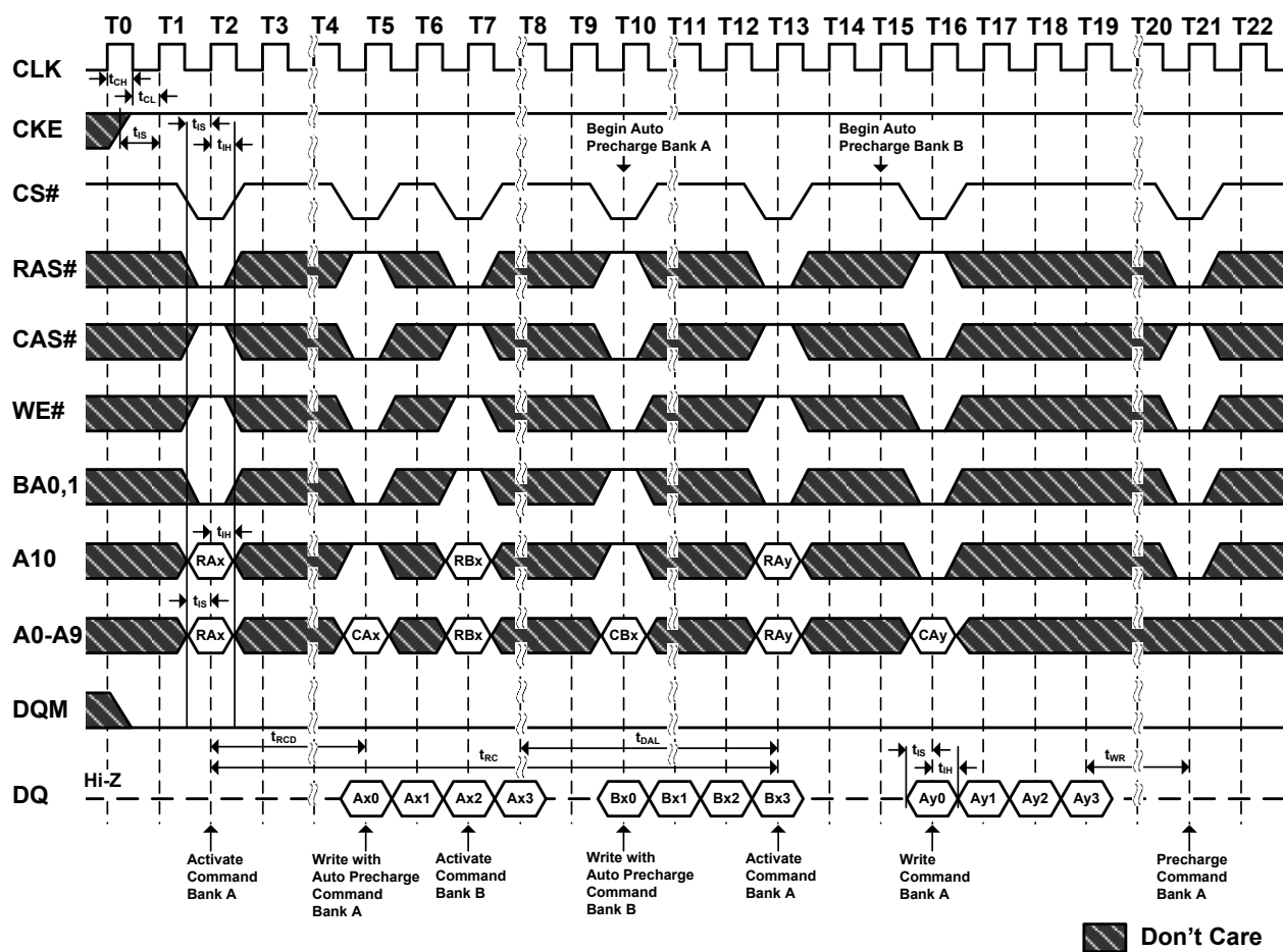
Figure 19. AC Parameters for Write Timing (Burst Length=4)
