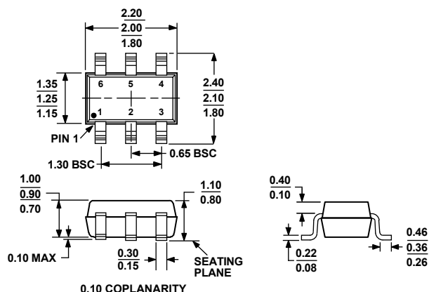
Figure 53. 6-Lead Thin Shrink Small Outline Transistor Package [SC70]
