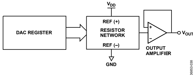
Figure 38. DAC Architecture
