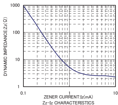
Z z -I Z CHARACTERISTICS
