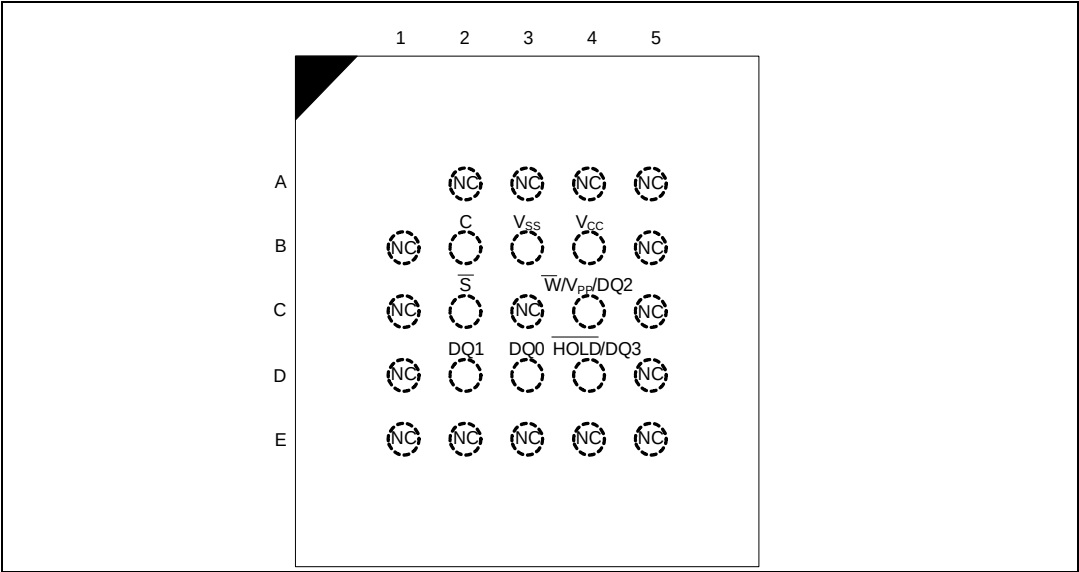
Figure 4. BGA connections
