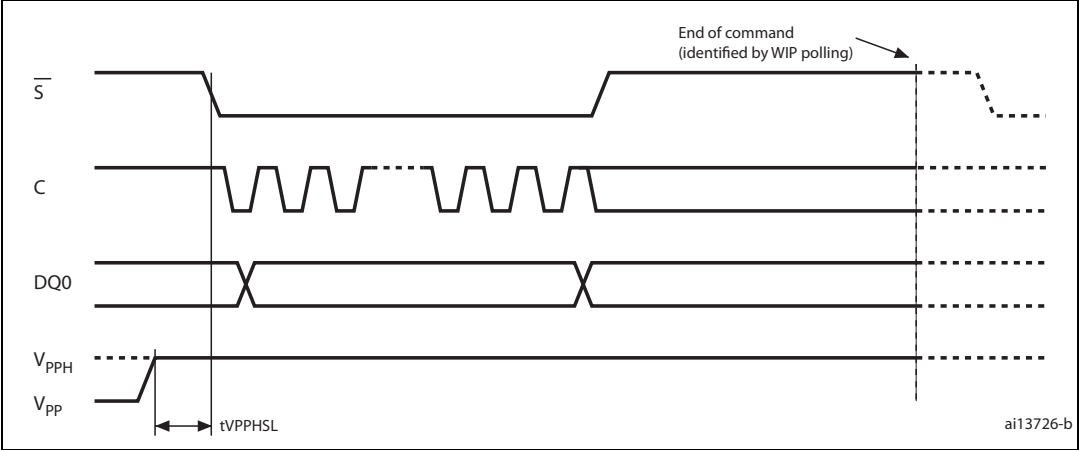
Figure 109. V_{PPH} timing
