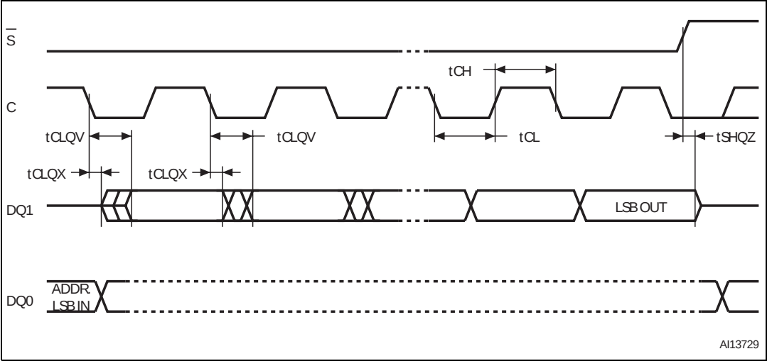
Figure 108. Output timing
