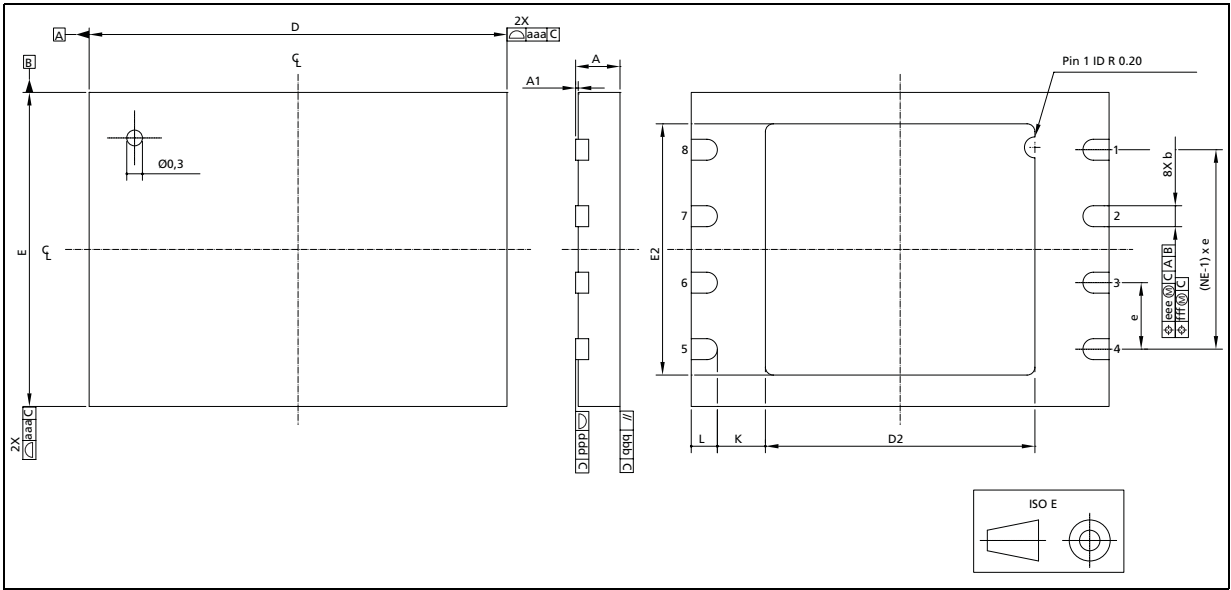
Figure 112. VDFPN8 (MLP8) Very Thin Dual Flat Package 8 leads, 8×6×1 mm Drawing
