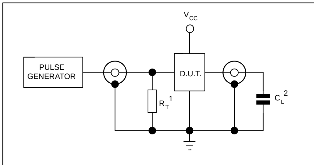
Figure 4: Test circuit
