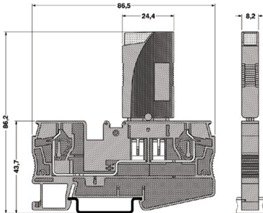
Dimensioned drawing
