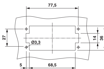
Dimensioned drawing
