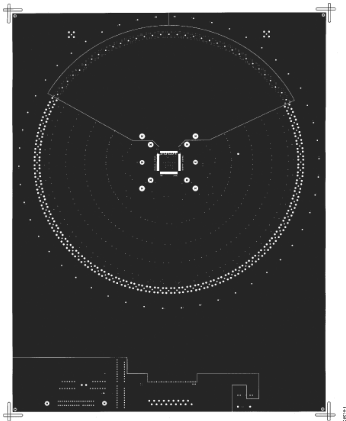
Figure 49. INT1 ( V_{EE} )
