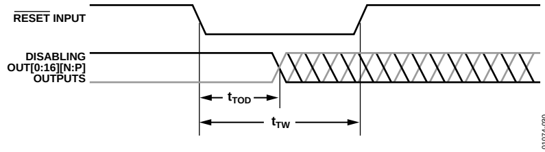
Figure 30, Asynchronous Reset
