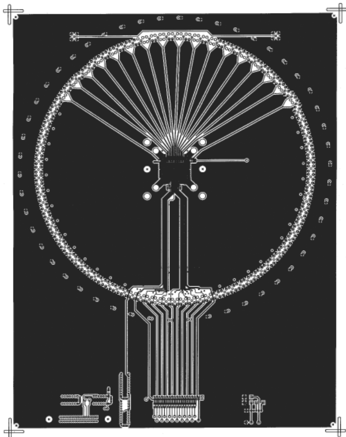
Figure 43. Component Side
