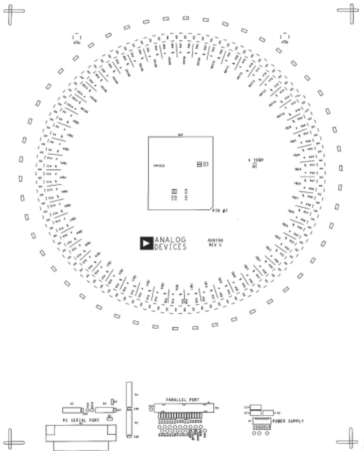
Figure 45. Silkscreen Top
