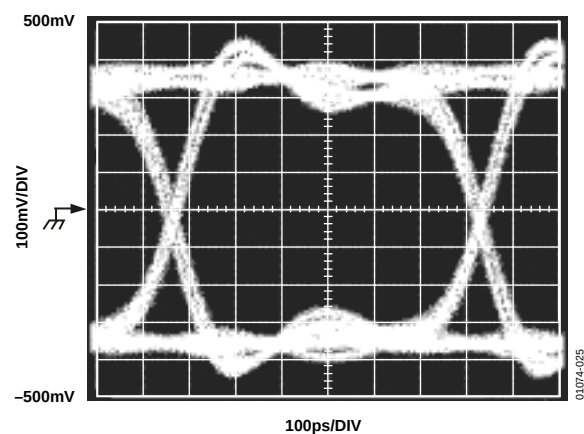
Figure 24. Eye Pattern, V_{EE} = -5\text{ V} , 1.5 Gbps PRBS 23
