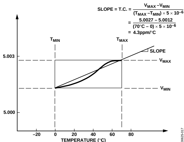
Figure 18. Typical AD586L Temperature Drift
