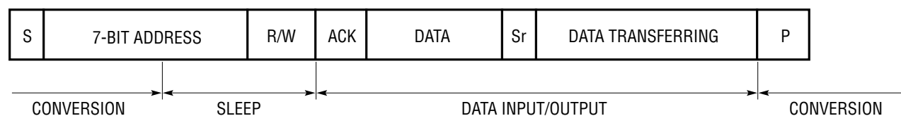
Figure 6. Conversion Sequence
