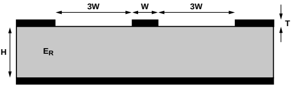
Figure 46. Cross-Sectional View of a PC Board
