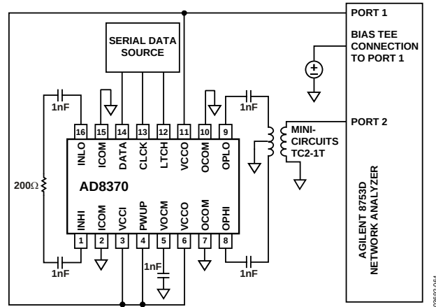
Figure 66. PSRR A_s Test Setup
