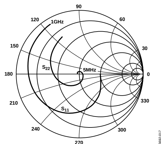
Figure 19. Input and Output Reflection Coefficients, S_{11} and S_{22} , Z_0 = 100\text{ }\Omega Differential
