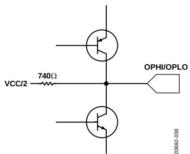
Figure 40. OPHI/OPLO Simplified Circuit
