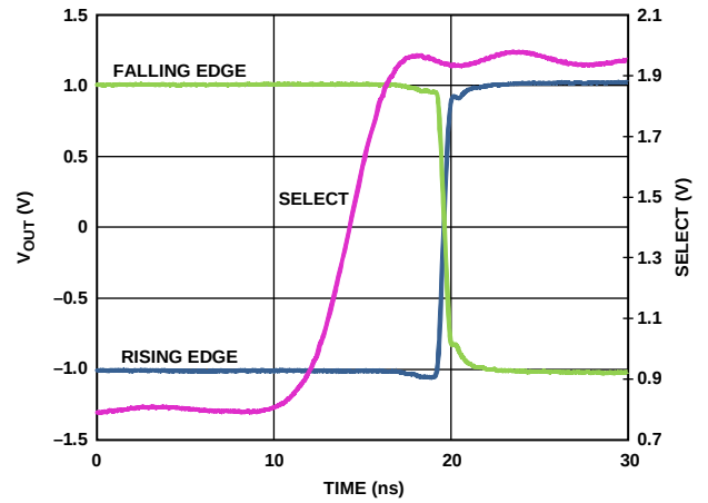
Figure 19. ADV3220 Switching Time
