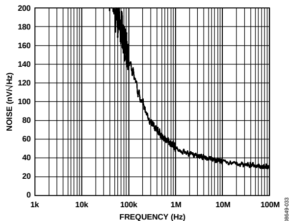
Figure 33. ADV3220 Noise vs. Frequency
