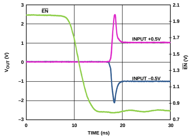
Figure 21. ADV3220 Enable On Timing
