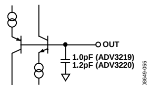
Figure 53. ADV3219/ADV3220 Disabled Output
