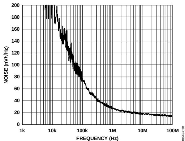
Figure 30. ADV3219 Noise vs. Frequency
