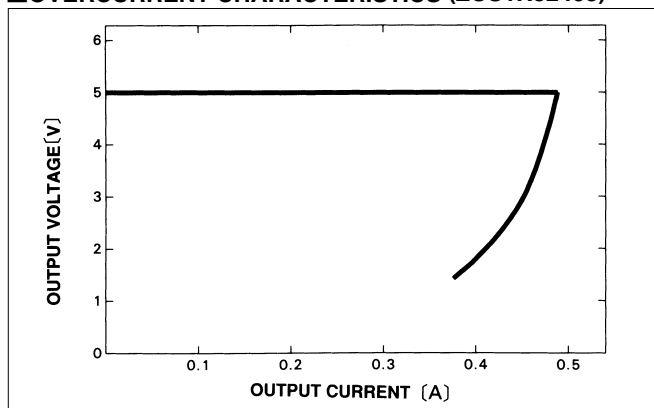
■ OVERCURRENT CHARACTERISTICS (ZUS1R52405)
