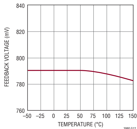
Feedback Voltage
