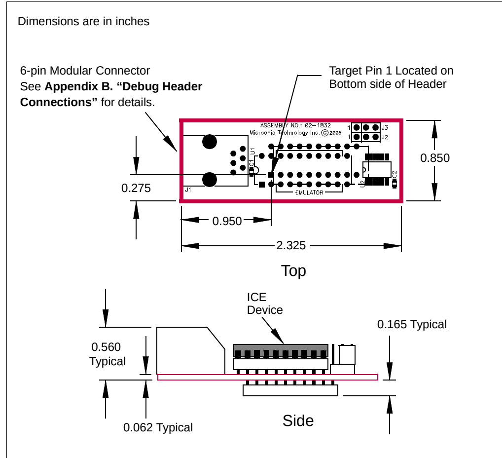
FIGURE 8: DIMENSIONS – AC162066
