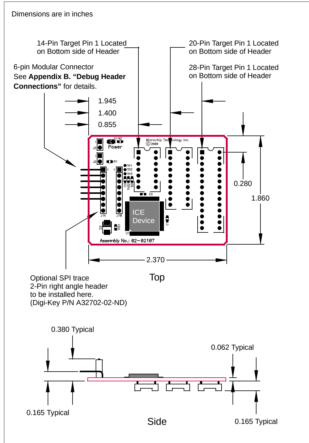
FIGURE 12: DIMENSIONS - AC244028
