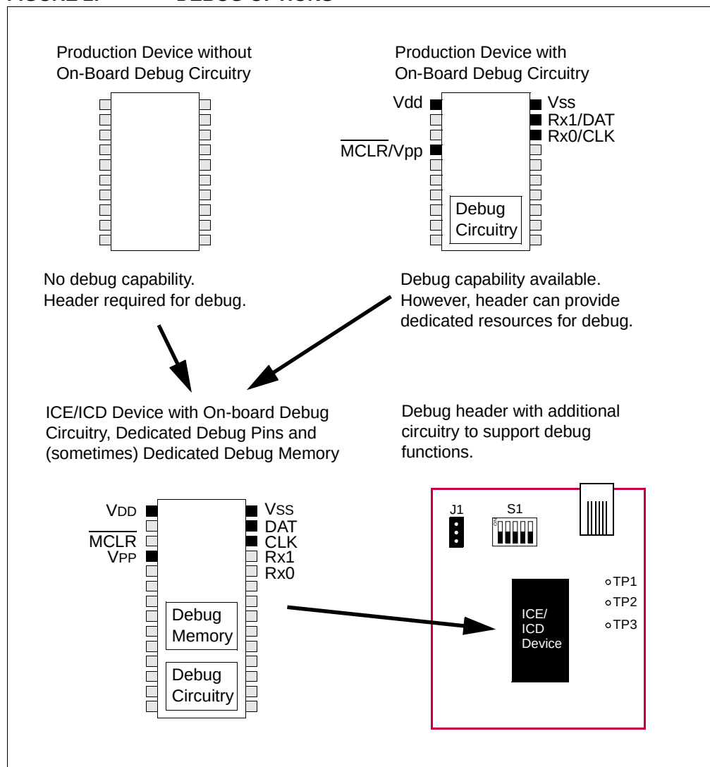
FIGURE 2: DEBUG OPTIONS
