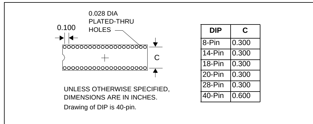
FIGURE 16: DIP FOOTPRINT
