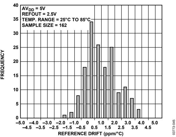
Figure 16. AD539x REFOUT Temperature Coefficient
