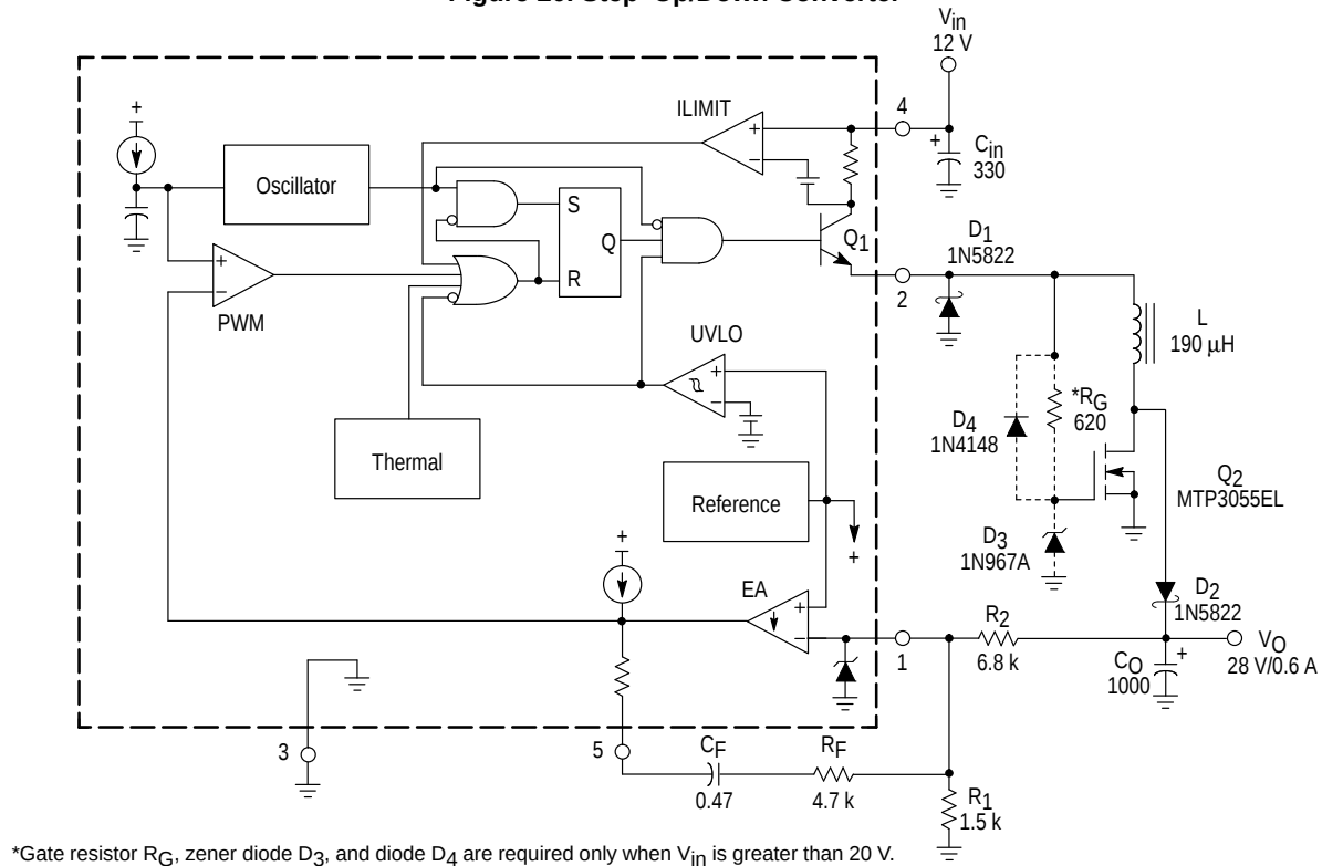
Figure 20. Step-Up/Down Converter
