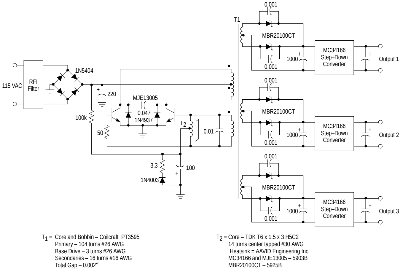
Figure 27. Off-Line Preconverter
