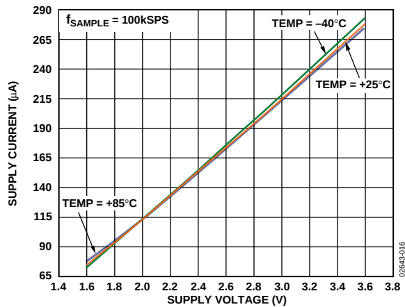
Figure 15. AD7466 Supply Current vs. Supply Voltage, SCLK 3.4 MHz
