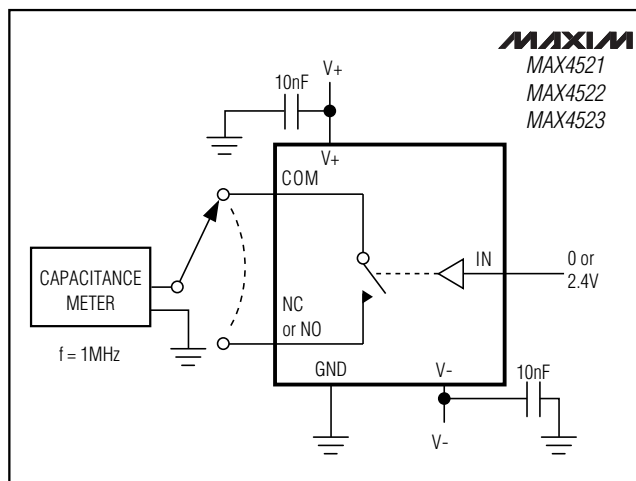
Figure 6. Channel Off-Capacitance
