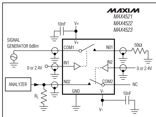
Figure 5. Crosstalk
