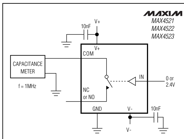
Figure 7. Channel On-Capacitance
