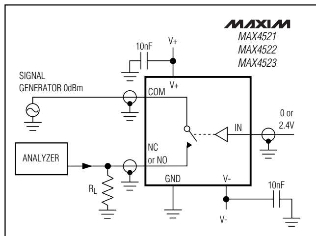
Figure 4. Off-Isolation
