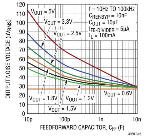
RMS Output Noise vs Feedforward Capacitor ( C_{\text{FF}} )
