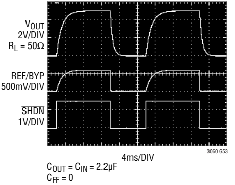
SHDN Transient Response C_{REF/BYP} = 10nF
