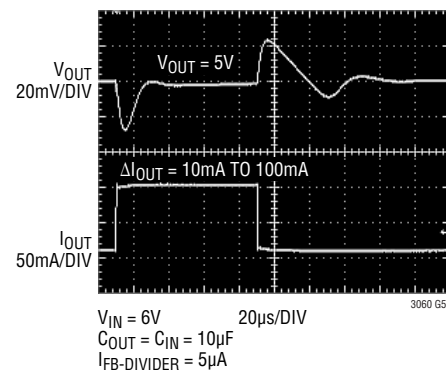
LT3060-5 Transient Response, C_{\text{FF}} = 10\text{nF}
