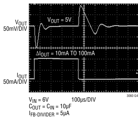
LT3060-5 Transient Response, C_{\text{FF}} = 0
