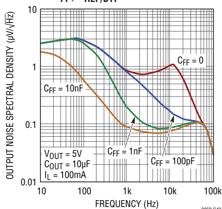
Output Noise Spectral Density vs C_{FF} , C_{REF/BYP} = 10nF
