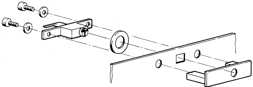
Blech-Frontplatte (Tastatureinschub)
