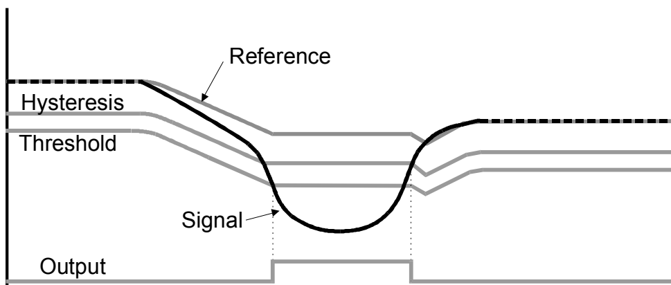
Figure 7-1. Thresholds and Drift Compensation
