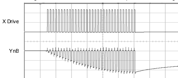
Figure 4-1. VCs – Nonlinear During Burst (Burst too long, or C_s too small, or X-Y transcapacitance too large)
