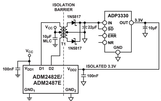
Figure 34. Applications Diagram
