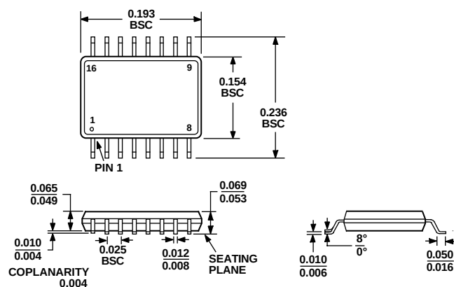
COMPLIANT TO JEDEC STANDARDS MO-137AB Figure 70. 16-Lead Shrink Small Outline Package [QSOP] (RQ-16) Dimensions in Inches
