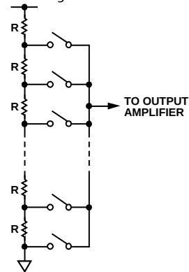
Figure 43. Resistor String
