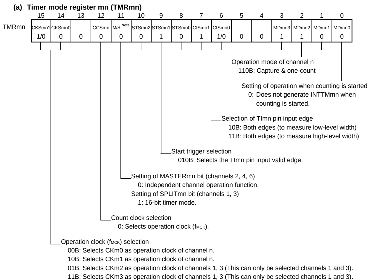
Figure 6-59. Example of Set Contents of Registers to Measure Input Signal High-/Low-Level Width
