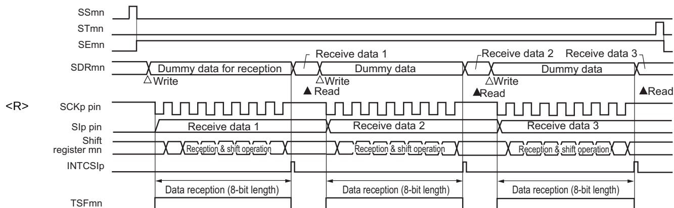
Figure 12-38. Timing Chart of Master Reception (in Single-Reception Mode)
