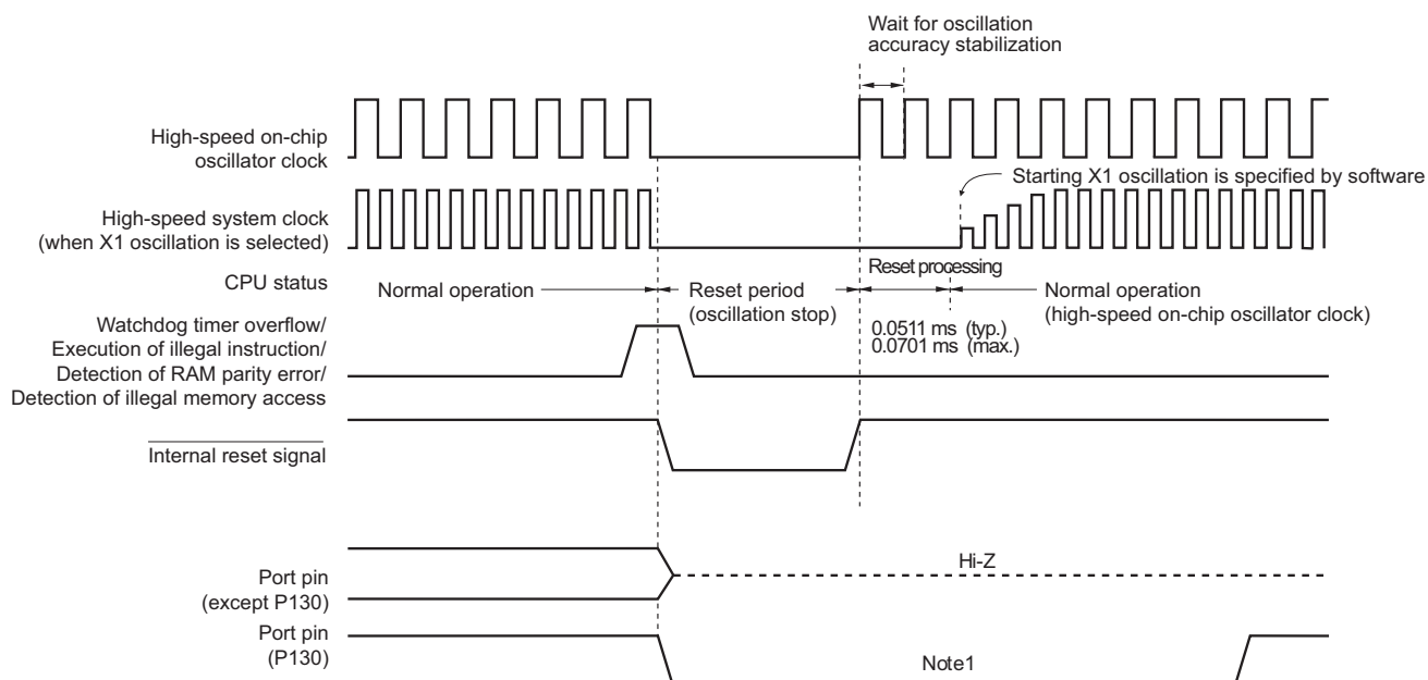
Figure 19-3. Timing of Reset Due to Execution of Illegal Instruction, Watchdog Timer Overflow, RAM Parity Error, or Illegal Memory Access
