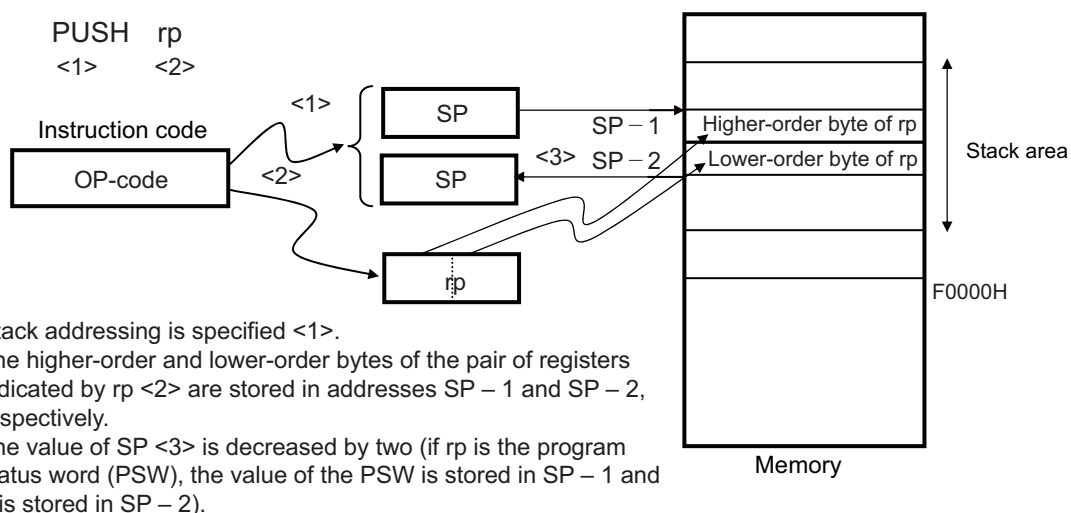
Figure 3-50. Example of PUSH rp
