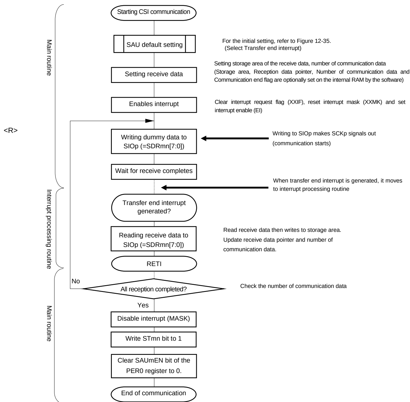
Figure 12-39. Flowchart of Master Reception (in Single-Reception Mode)
