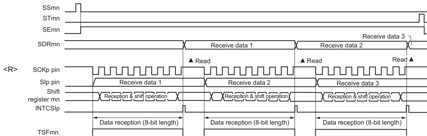
Figure 12-62. Timing Chart of Slave Reception (in Single-Reception Mode)
