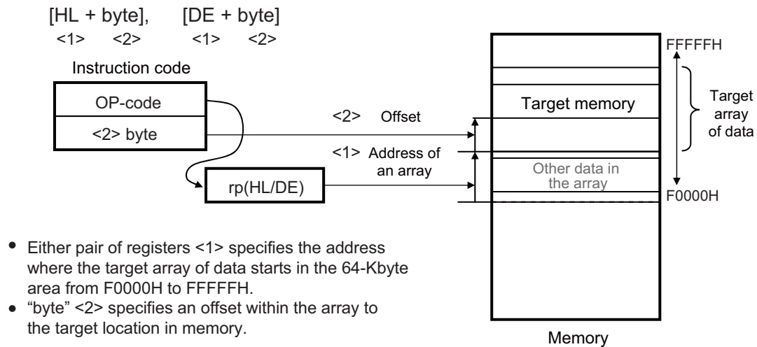
Figure 3-42. Example of [HL+byte], [DE+byte]
