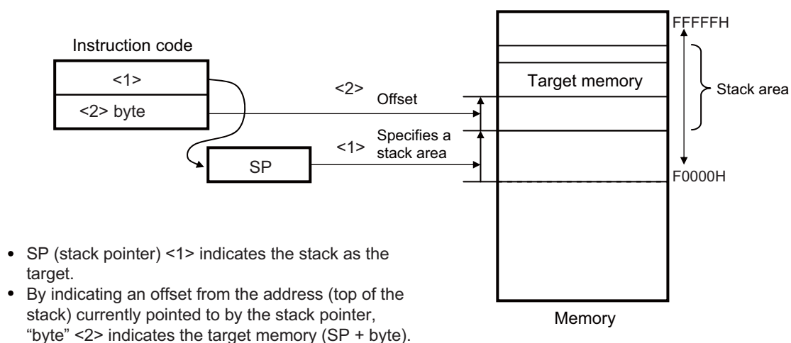
Figure 3-41. Example of [SP+byte]
