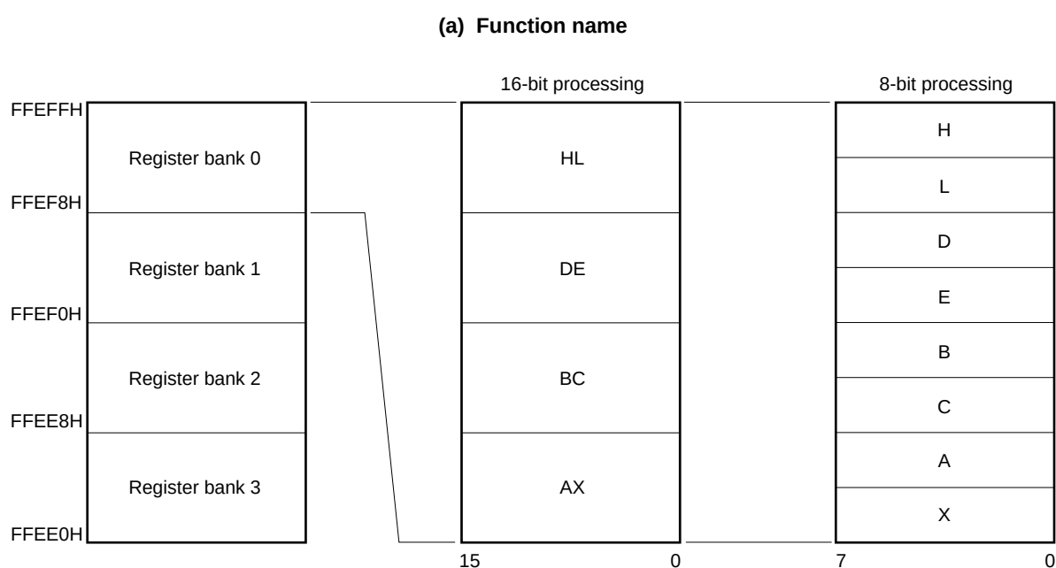
Figure 3-25. Configuration of General-Purpose Registers
