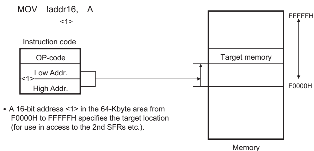
<R> Figure 3-35. Example of !addr16
