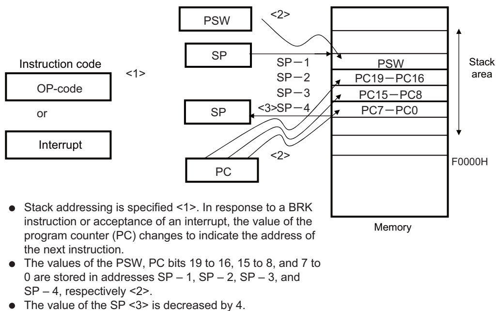
Figure 3-54. Example of Interrupt, BRK
