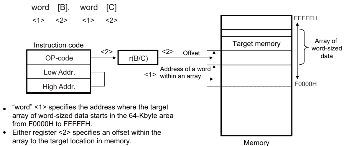
Figure 3-43. Example of word[B], word[C]
