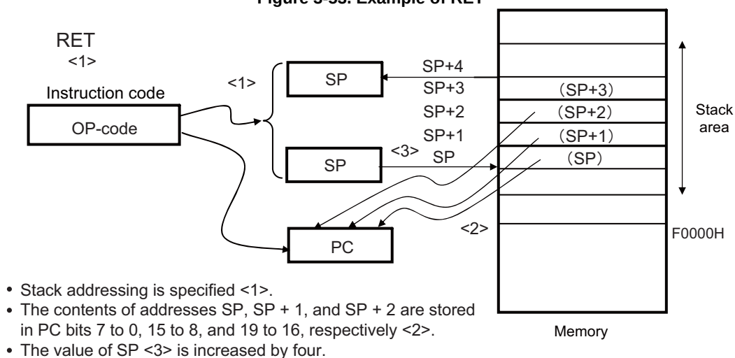
Figure 3-53. Example of RET
