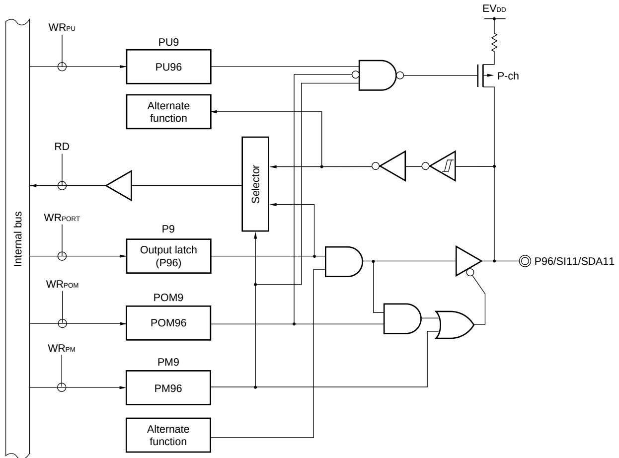
Figure 4-44. Block Diagram of P96
