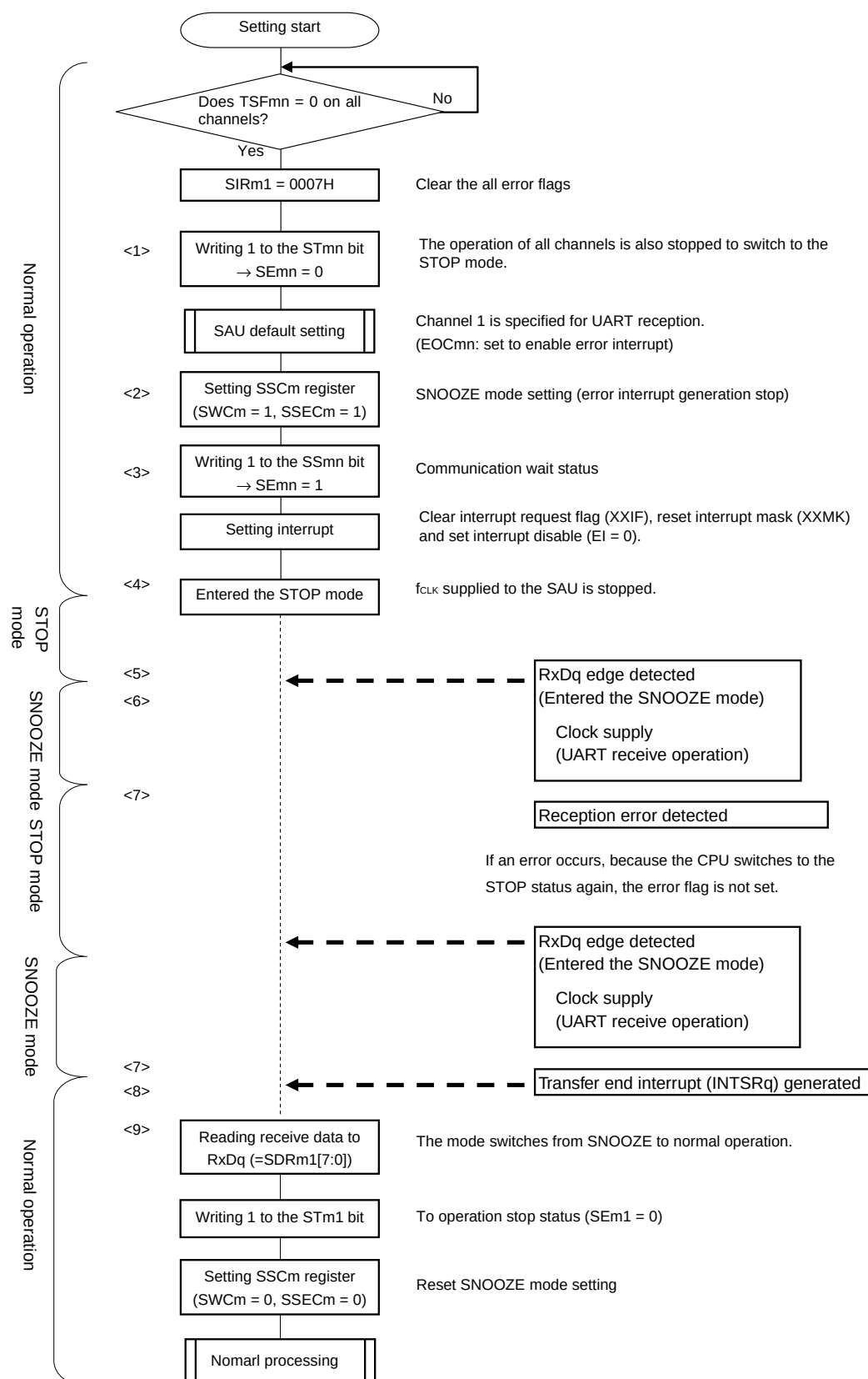
Figure 12-95. Flowchart of SNOOZE Mode Operation (Abnormal Operation &lt;2&gt;)
