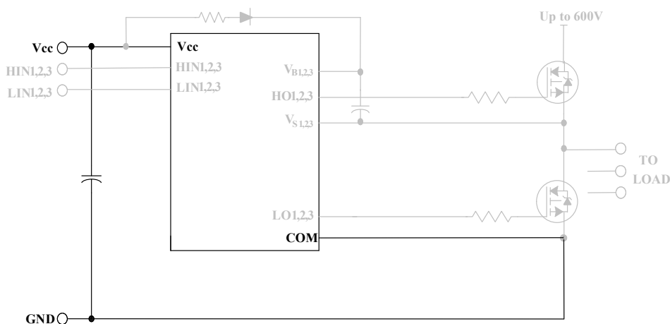
Figure 21: Supply capacitor
