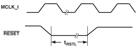
Figure 2. RESET Timing
