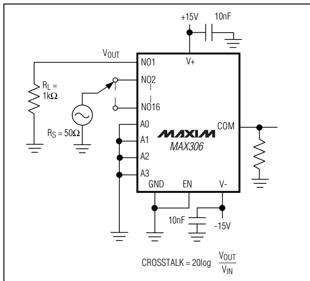
Figure 7. Crosstalk
