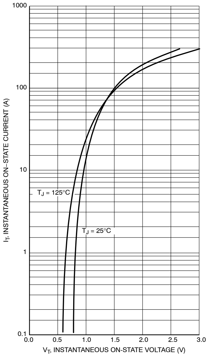
Figure 3. On-State Characteristics
