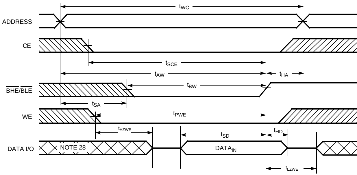
Figure 10. Write Cycle No. 4 ( \overline{\text{BHE/BL E}} controlled, \overline{\text{OE}} LOW) [26]
