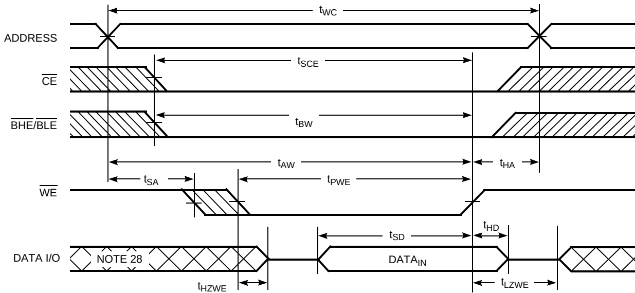
Figure 10. Write Cycle No. 4 ( \overline{\text{BHE/BL E}} controlled, \overline{\text{OE}} LOW) [26]
