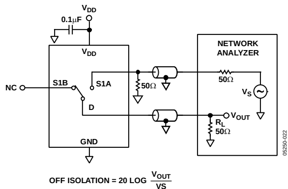
Figure 34. Off Isolation
