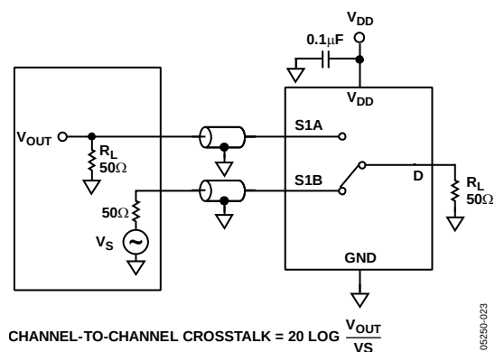
Figure 35. Channel-to-Channel Crosstalk (S1A to S1B)
