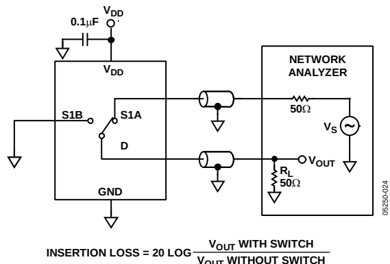
Figure 36. Bandwidth
